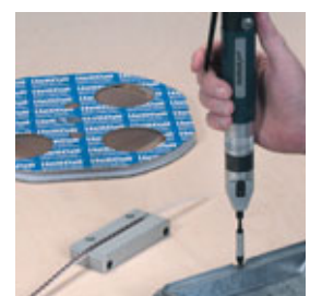
Installation of HELICOIL® plus
