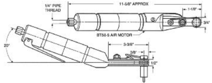
20° Offset Ratchet Wrench Driver Assembly With Multi-Length Socket And Super Key (T-Series)
